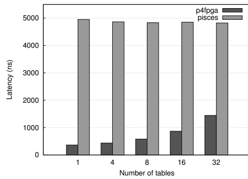
Figure 8: Processing latency v.s. number of tables
